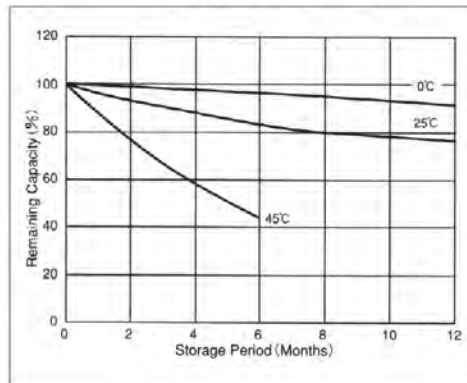
Self-discharge Characteristics
