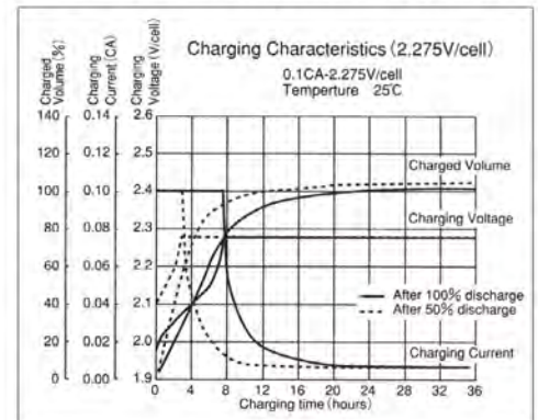
Charging Characteristics(2.275V/cell)
